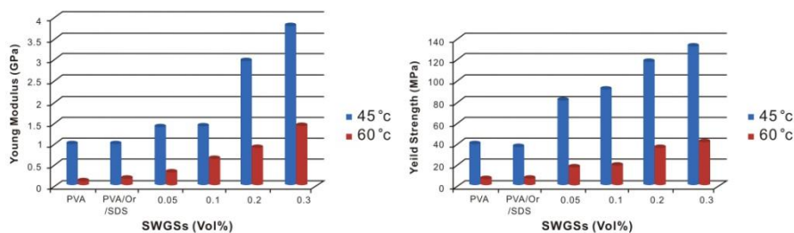
Fig. 3.13 Comparison between mechanical properties of the prepared samples at 45 and 60 °C.
